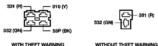
RIGHT POWER DOOR LOCK MOTOR
