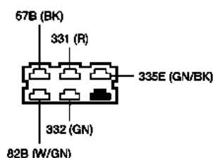
POWER DOOR LOCK RELAY
