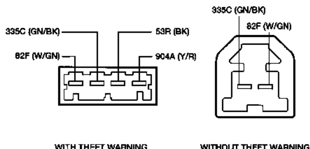
RIGHT POWER KEY LOCK SWITCH
