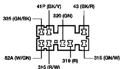
RIGHT POWER DOOR LOCK SWITCH
