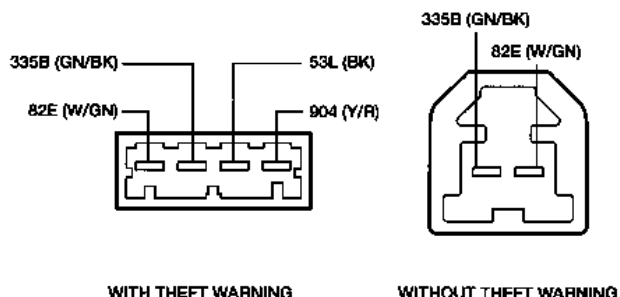
LEFT POWER KEY LOCK SWITCH
